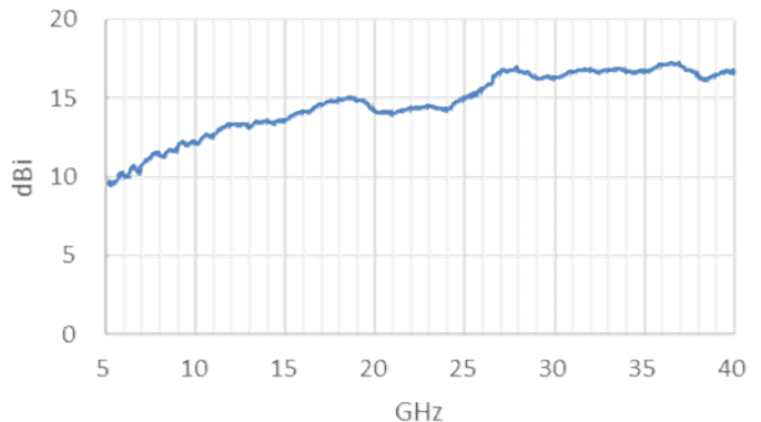
Gain(typ.)
